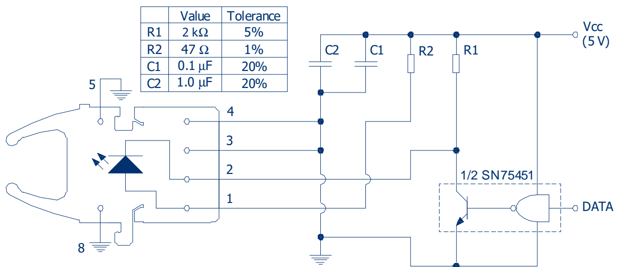
FIGURE 2 Recommended transmitter application circuit. See note 7 Table 6
